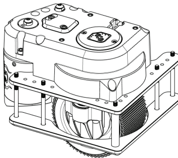
MK5n Compact layout
